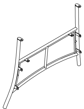
A x 2 Legs
